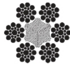
6x19S
