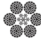
6x36WS Dycam
